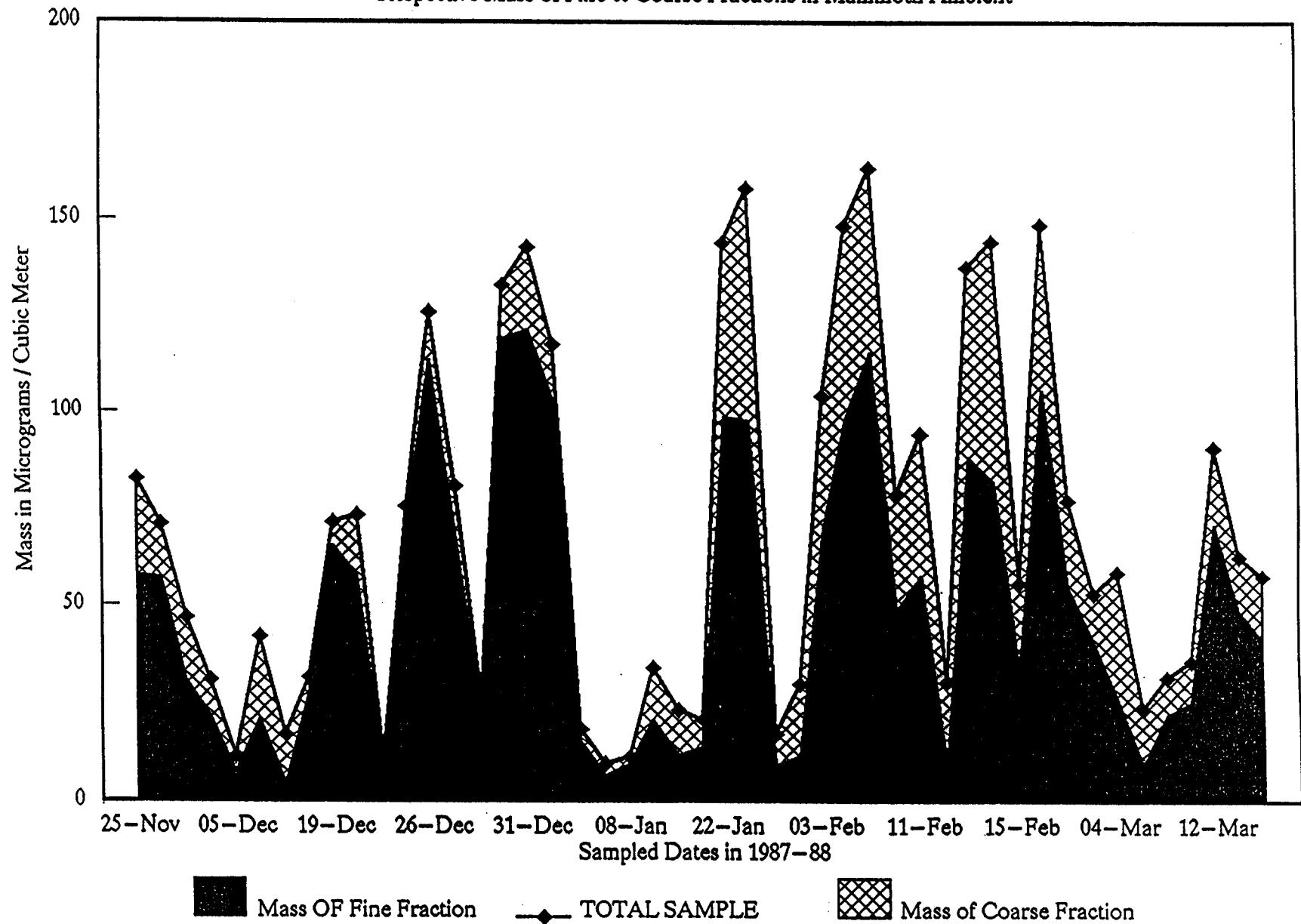
FIGURE 4.1 Respective Mass of Fine & Coarse Fractions in Mammoth Ambient
