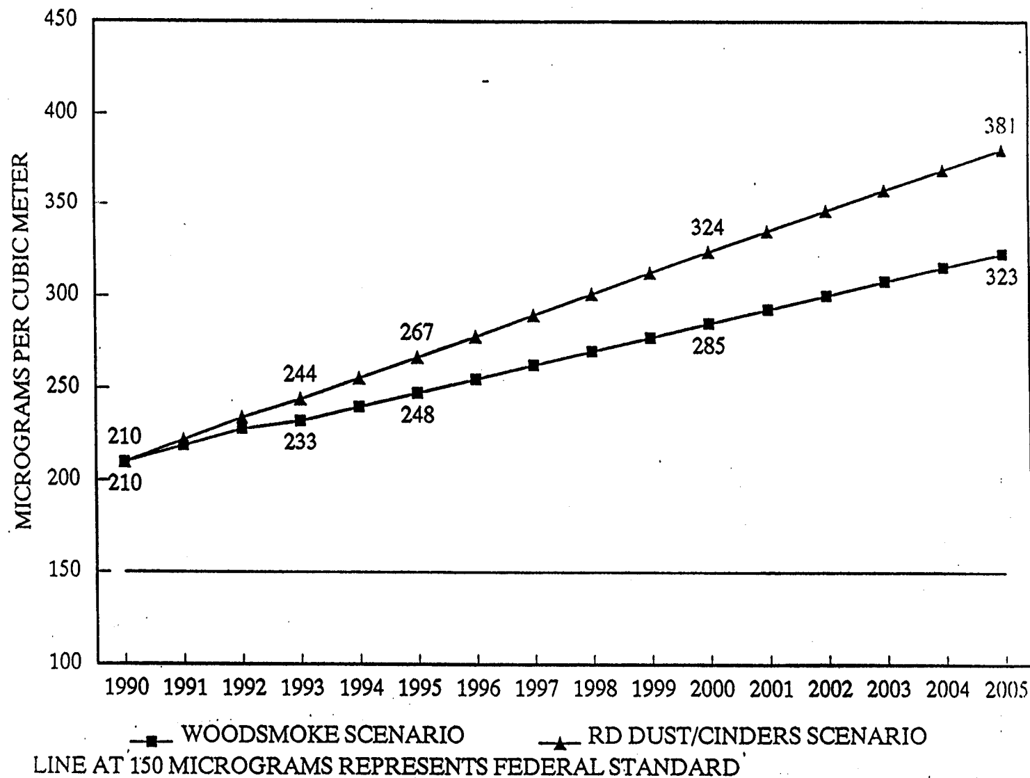
FIGURE 5.1 FORECASTED AIR QUALITY - UNCONTROLLED
